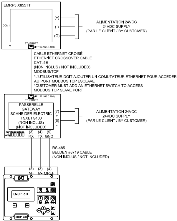
EMRP3.X855TT CONFIGURATION DE BASE BASIC SETUP
