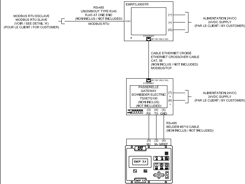
EMRP3.X855TR CONFIGURATION DE BASE BASIC SETUP
